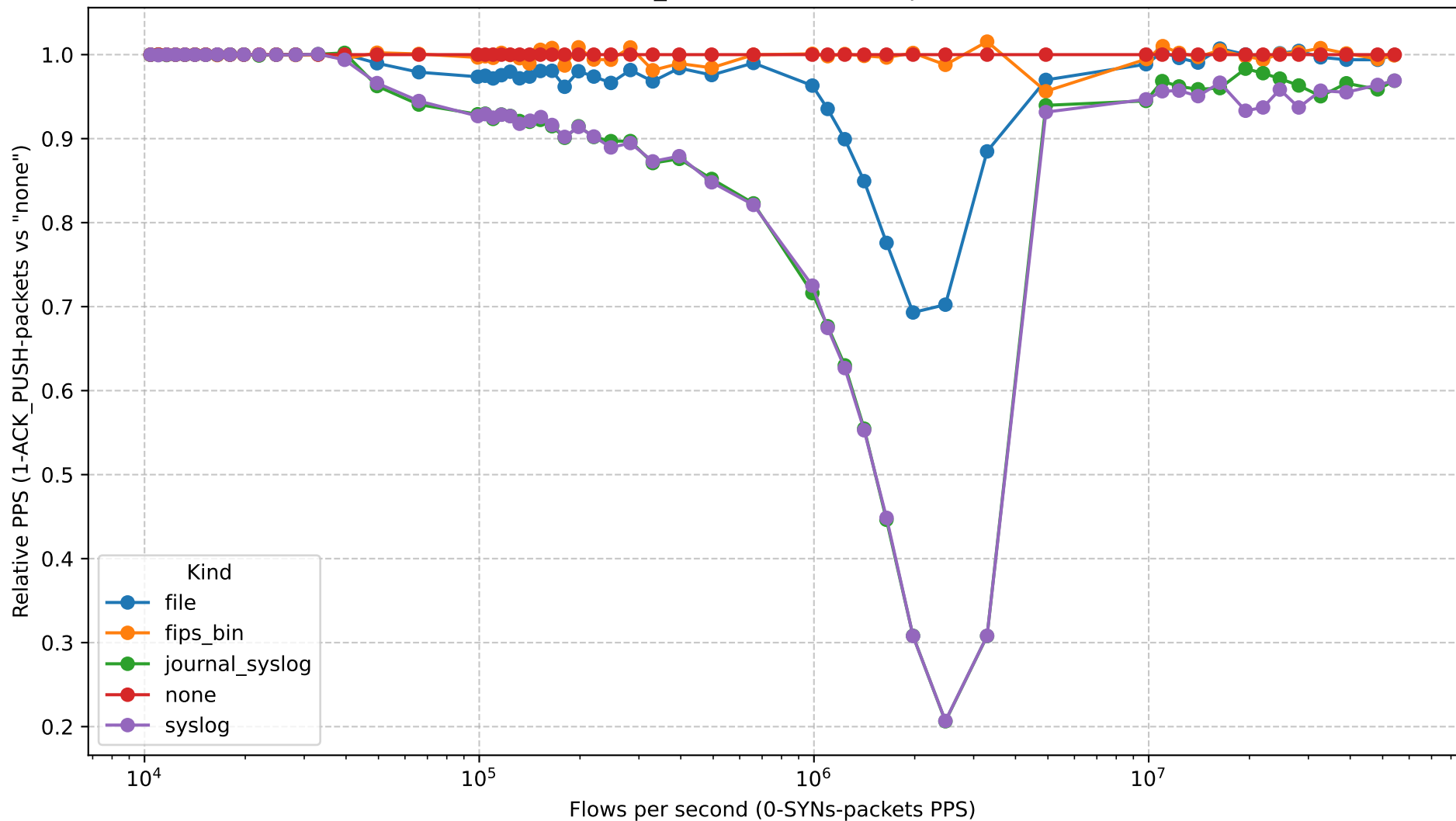
Relative ACK_PUSH PPS vs Flows per Second
