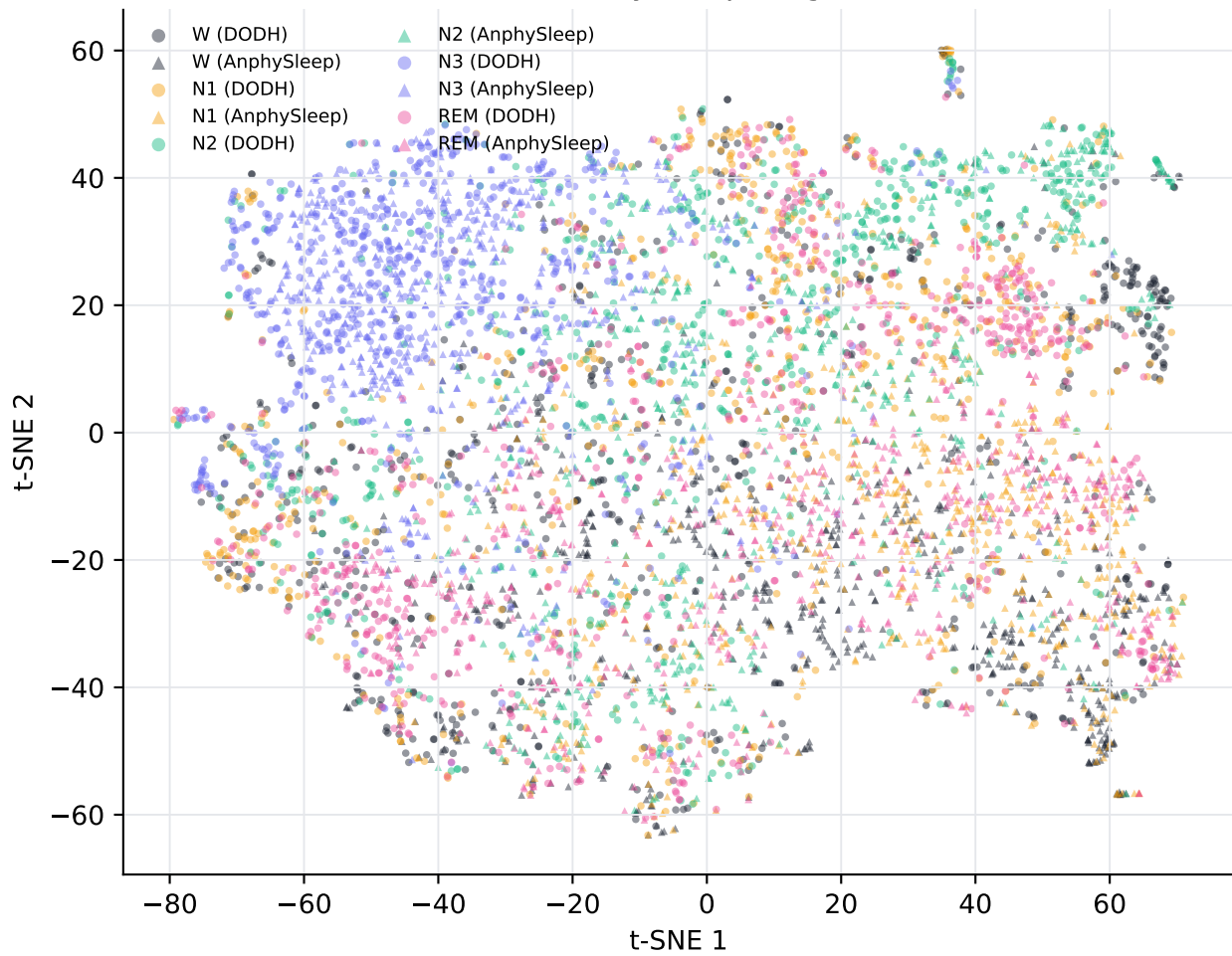
t-SNE by sleep stage
