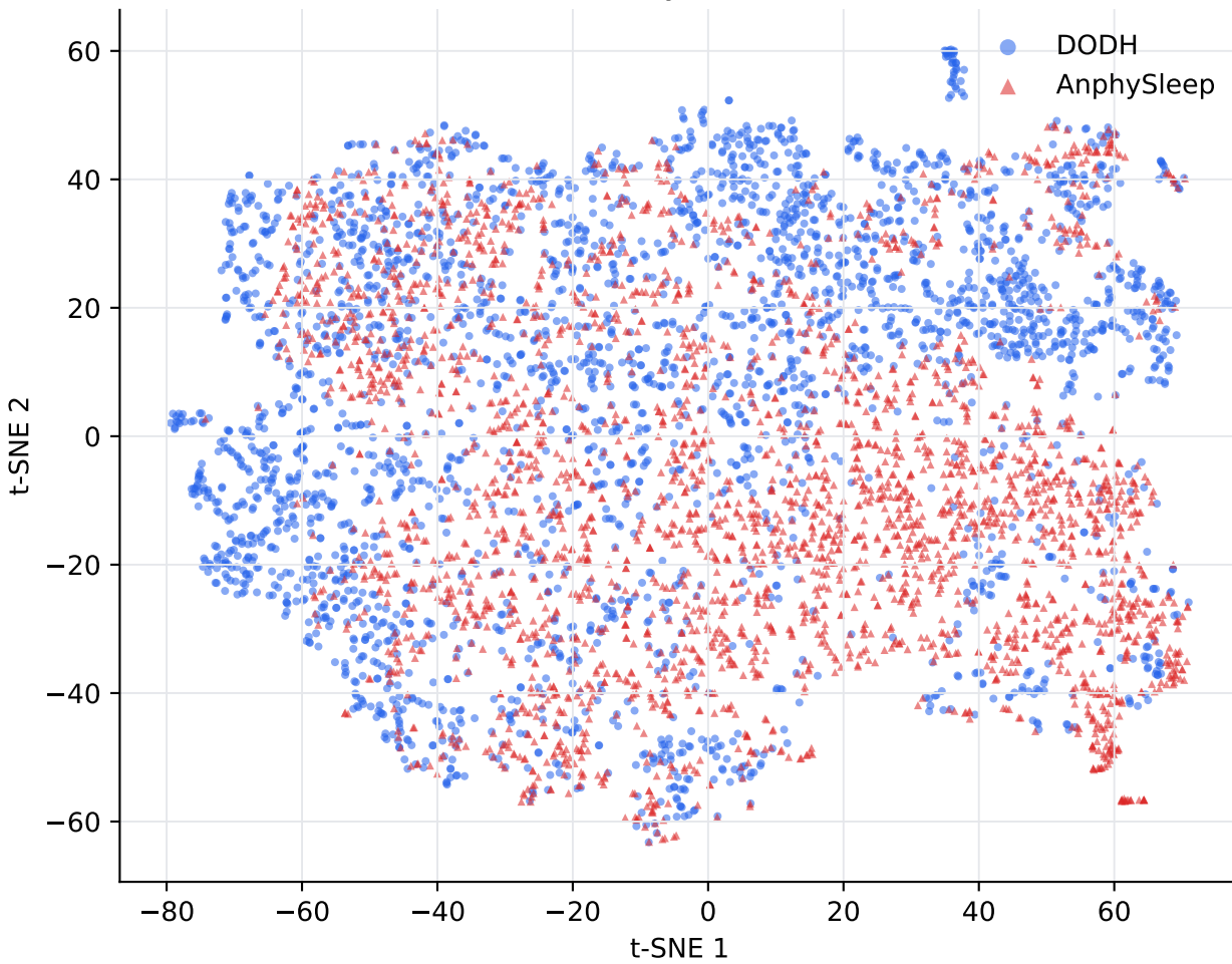
t-SNE by dataset
