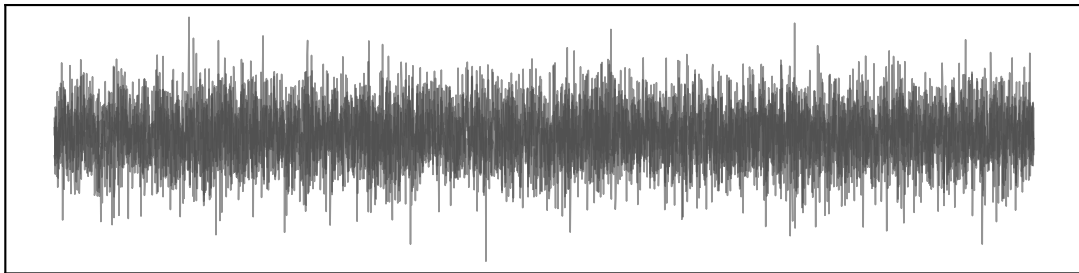
Node activity
