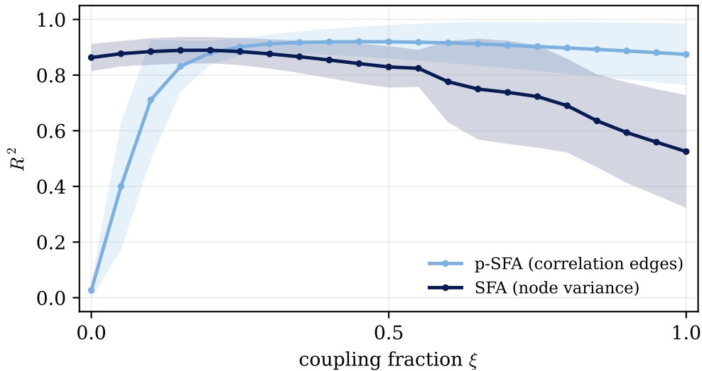
TVP Recovery along the variance \leftrightarrow coupling path
