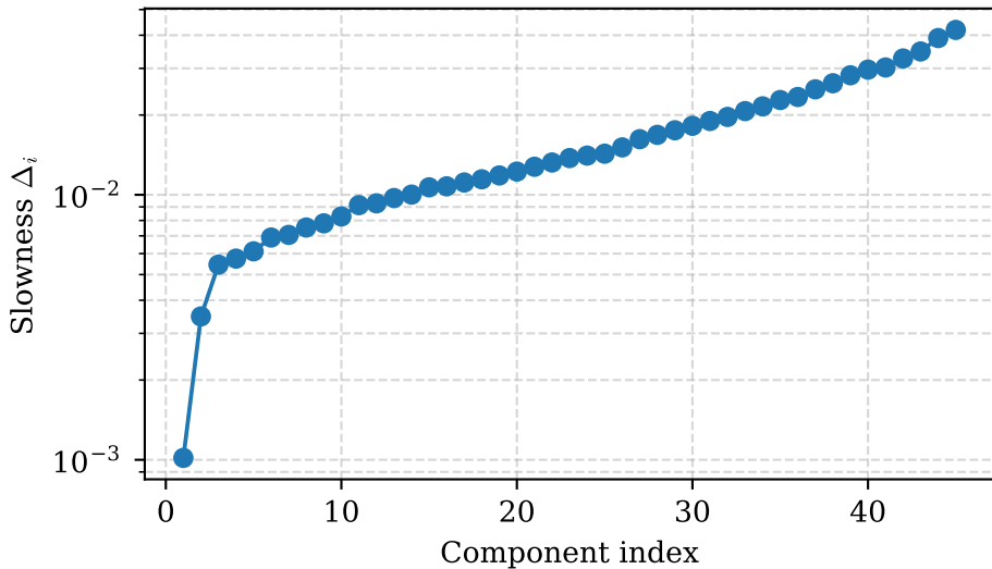
SFA slowness spectrum
