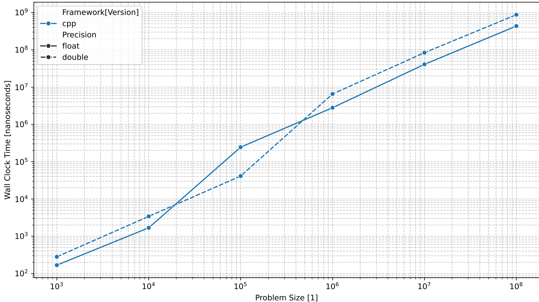
Runtime in nanoseconds vs. Problem Size N for VecAdd
