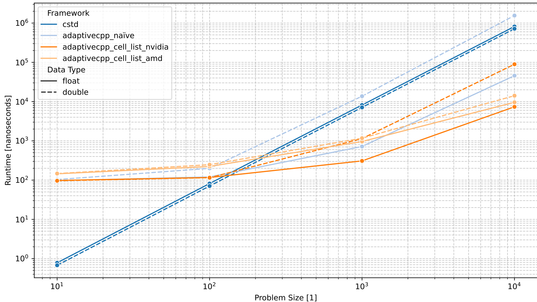
Runtime in nanoseconds vs. Problem Size N for NBody
