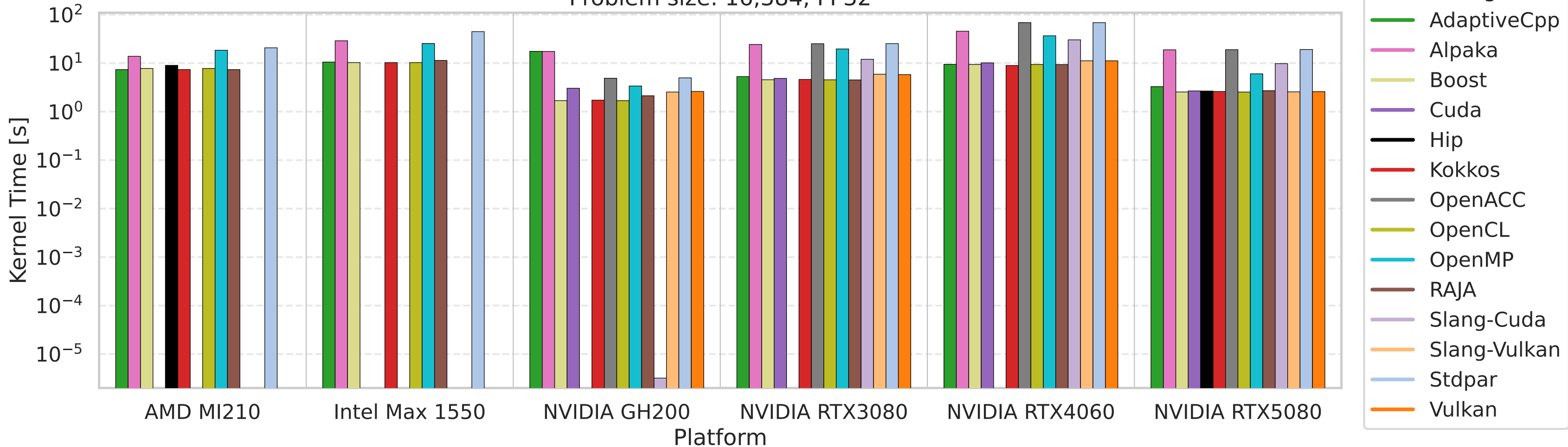
MatrixMultiplication Kernel Time Problem size: 16,384, FP32
