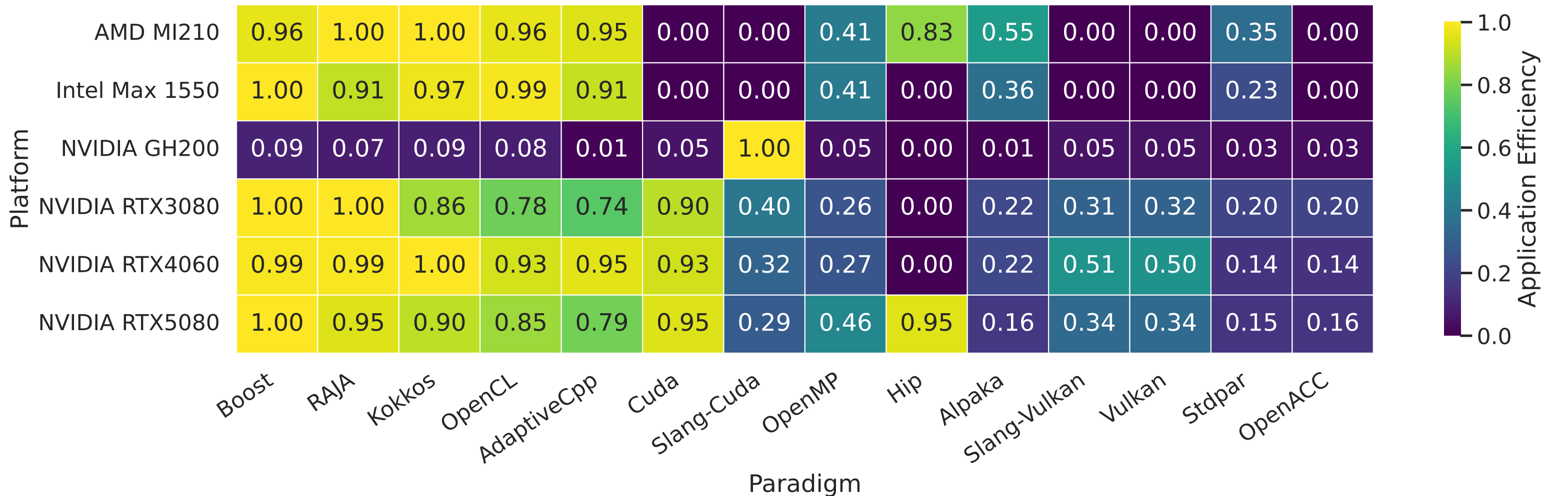
MatrixMultiplication Application Efficiency Heatmap Problem size: 16384
