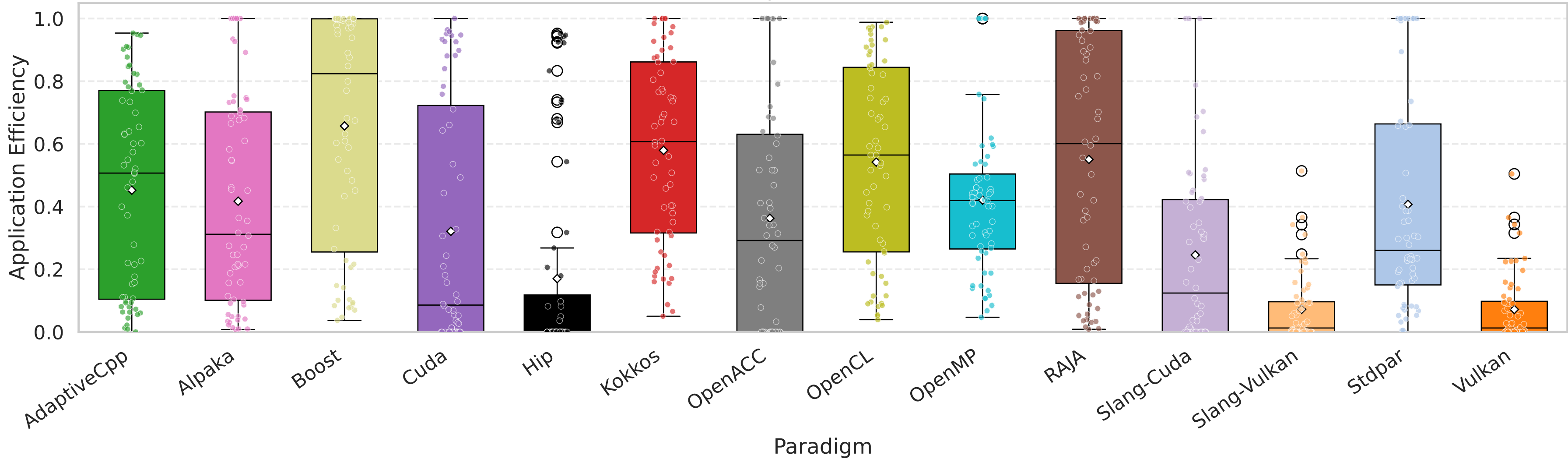
MatrixMultiplication Application Efficiency by Paradigm All problem sizes
