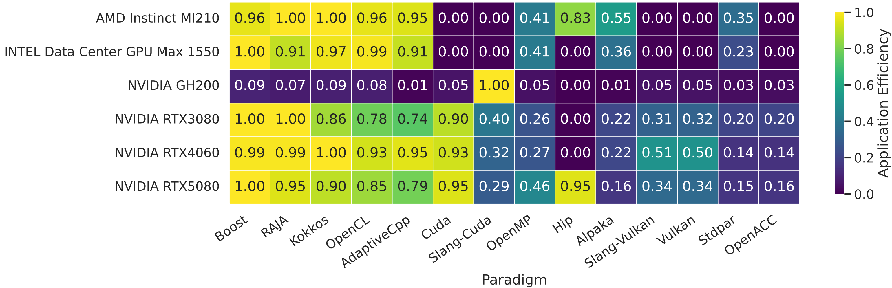
MatrixMultiplication Application Efficiency Heatmap
