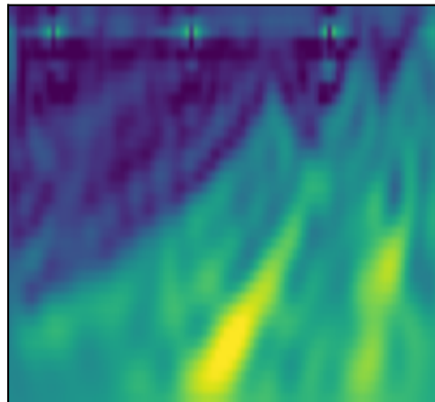
10 dB final RMSE 182.6 m/s, SSIM 0.514
