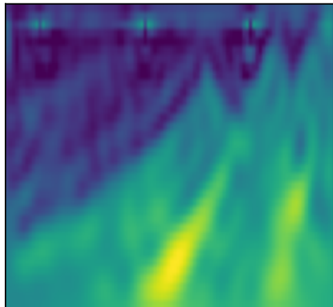
10 dB selected RMSE 180.3 m/s, SSIM 0.520
