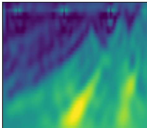
left-center: selected RMSE 184.4 m/s, SSIM 0.500
