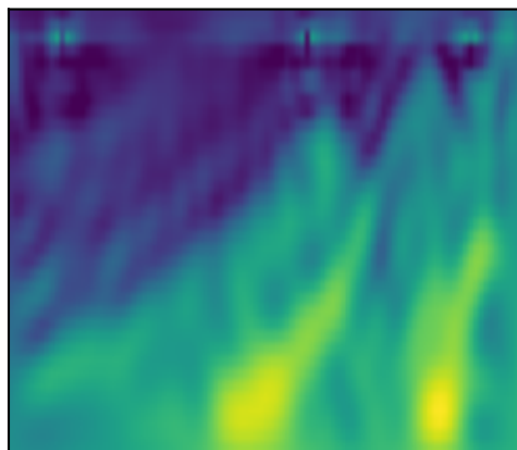
outer-inner: selected RMSE 177.5 m/s, SSIM 0.521
