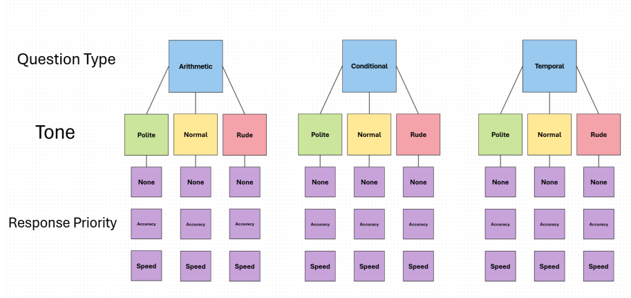
Figure 1: Structure of LLM Prompting Design
