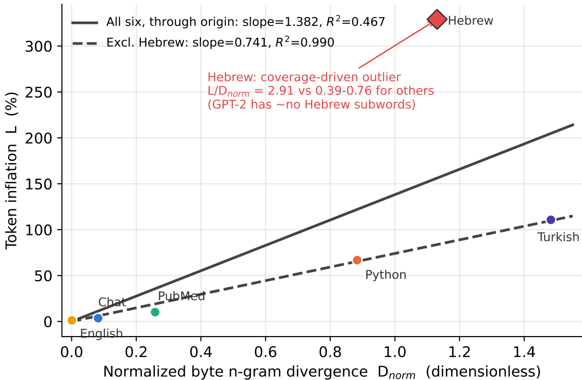
Token inflation vs distributional divergence (test split, seed 0)
