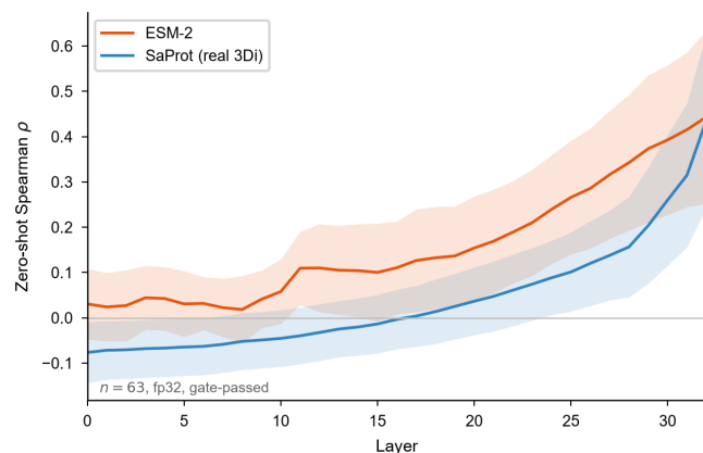
Figure 4 Logit lens: zero-shot mutation scoring by layer ( n = 63 ). Both models improve with depth and attain their maximum at the final layer: ESM-2 (orange) rises from \rho = 0.03 (layer 0) to \rho = 0.443 (layer 32); SaProt with real 3Di tokens (blue) rises from negative early-layer values to \rho = 0.437 (layer 32). Shaded bands indicate \pm 1 standard deviation across datasets. All computations in fp32 and validated against the official logits pathway.
