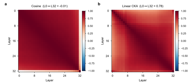
Figure 2 Layer-wise similarity matrices for SaProt ( 33 \times 33 ). Averaged over 10 datasets and 200 random residue positions per dataset. (a) Cosine: adjacent layers are highly similar ( \cos \approx 0.98 ); mean similarity decays monotonically with distance and collapses to -0.01 only between the most distant layers (Layer 0 vs. 32). (b) Linear CKA over the same hidden states: the most distant layers retain CKA 0.81, indicating a rotation that preserves linearly decodable information rather than information loss.
