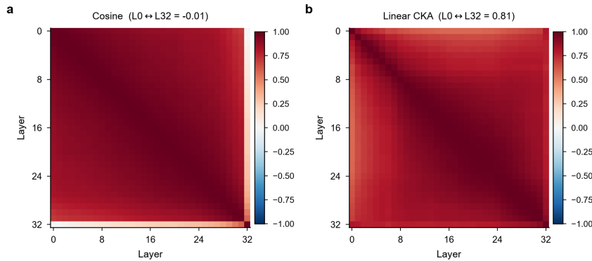
Figure 2: Layer-wise similarity matrices for SaProt (33×33). Averaged over 10 datasets and 50 random residue positions per dataset. (a) Cosine: adjacent layers are highly similar ( \cos = 0.98 ); mean similarity decays monotonically with distance and collapses to -0.01 only between the most distant layers (Layer 0 vs. 32). (b) Linear CKA over the same hidden states: the most distant layers retain CKA 0.81, indicating a rotation that preserves linearly decodable information rather than information loss.
