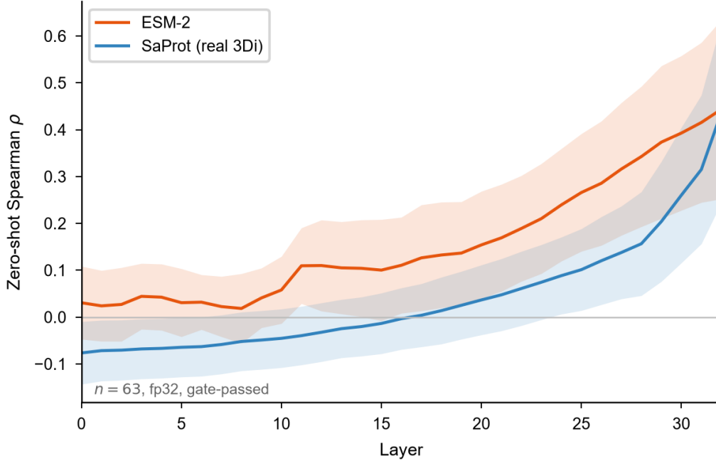
Figure 4: Logit lens: zero-shot mutation scoring by layer ( n = 63 ). Both models improve with depth and attain their maximum at the final layer: ESM-2 (orange) rises from \rho = 0.03 (layer 0) to \rho = 0.443 (layer 32); SaProt with real 3Di tokens (blue) rises from negative early-layer values to \rho = 0.437 (layer 32). Shaded bands indicate \pm 1 standard deviation across datasets. All computations in fp32 and validated against the official logits pathway; the previously reported non-monotonic ESM-2 curve is withdrawn.
