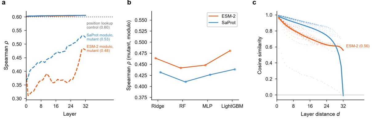
Figure 3: Per-layer probing, multi-scale pooling, and layer distance under the unified protocol. (a) 33-layer probing (combined features): under the random split the masked-arm profile is flat for both models ( \sigma \approx 10^{-3} ) and is reproduced by the random-position lookup control (dotted, 0.600); under leakage-free splits (modulo, mutant arm) performance is lower and the best layers are consistently late (layers 30–32, \Delta\rho \leq 0.009 versus the final layer). (b) Pooling (mutant arm, modulo split, 20 datasets per model; four strategies as dots, mean connected): ESM-2 spread across strategies 0.041 (Ridge) to 0.057 (RF); SaProt spread 0.005 (Ridge) to 0.039 (MLP); last-layer LightGBM is the best single configuration; per-fold-trained attention pooling is never best. (c) Cosine similarity versus layer distance (unique layer pairs): SaProt decays monotonically and reaches -0.01 only at the largest distances, while ESM-2 remains positive; linear CKA between the most distant SaProt layers remains 0.81 (Figure 2), indicating rotation with preserved linear information rather than loss.
