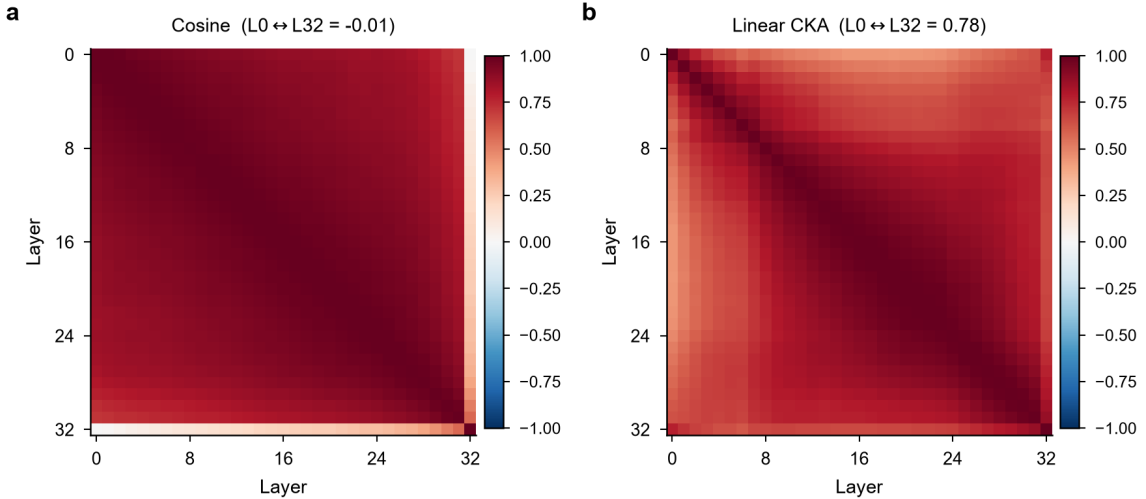
Figure 2: Layer-wise similarity matrices for SaProt (33×33). Averaged over 10 datasets and 200 random residue positions per dataset. (a) Cosine: adjacent layers are highly similar ( \cos = 0.98 ); mean similarity decays monotonically with distance and collapses to -0.01 only between the most distant layers (Layer 0 vs. 32). (b) Linear CKA over the same hidden states: the most distant layers retain CKA 0.81, indicating a rotation that preserves linearly decodable information rather than information loss.
