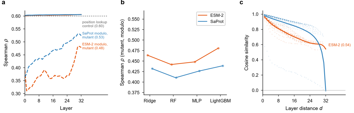
Figure 3: Per-layer probing, multi-scale pooling, and layer distance under a single fixed protocol. (a) 33-layer probing (combined features): under the random split the masked-arm profile is flat for both models ( \sigma \approx 10^{-3} ) and is reproduced by the random-position lookup control (dotted, 0.600); under leakage-free splits (modulo, mutant arm) performance is lower and the best layers are consistently late (layers 30–32, \Delta\rho \leq 0.009 versus the final layer). (b) Pooling (mutant arm, modulo split, 20 datasets per model; four strategies as dots, mean connected): ESM-2 spread across strategies 0.041 (Ridge) to 0.057 (RF); SaProt spread 0.005 (Ridge) to 0.039 (MLP); last-layer LightGBM is the best single configuration; per-fold-trained attention pooling is never best. (c) Cosine similarity versus layer distance (unique layer pairs): SaProt decays monotonically and reaches -0.01 only at the largest distances, while ESM-2 remains positive; linear CKA between the most distant SaProt layers remains 0.81 (Figure 2), indicating rotation with preserved linear information rather than loss.
