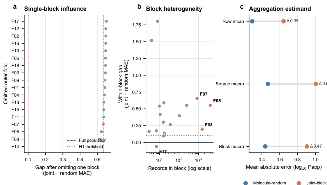
Figure S1: H1 influence and aggregation sensitivity. a , The D0 source-macro mean absolute error (MAE) gap between joint-block and molecule-random evaluation after omitting each of the 18 frozen joint blocks in turn. Points are ordered by the recalculated gap and labelled by the omitted outer fold. The black dashed line marks the full-population gap (0.537 \log_{10} Papp units), and the red dotted line marks the preregistered 0.10 point-gap threshold. Orange points identify omission of one of the three largest blocks. b , Within-block source-macro gap versus frozen block record count for all 18 blocks. The three largest blocks and the sole block with a negative within-block gap are labelled. The x axis is logarithmic; the red dotted line marks a gap of 0.10. c , Five-seed mean D0 MAE under row-micro, source-macro and equal-block-macro aggregation. Blue and orange points denote molecule-random and joint-block evaluation, respectively, and connecting segments show the corresponding gap. All panels use the already frozen 6,895-record, 41-source prediction population across five scheduled seeds. These post-confirmatory analyses involved no refitting or model selection and are descriptive; the original block/seed bootstrap remains the inferential H1 analysis.
