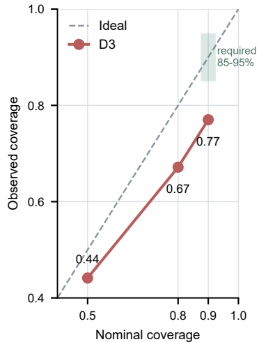
c D3 intervals are under-covered
