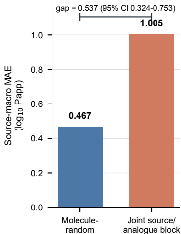
a Evaluation estimates diverge
