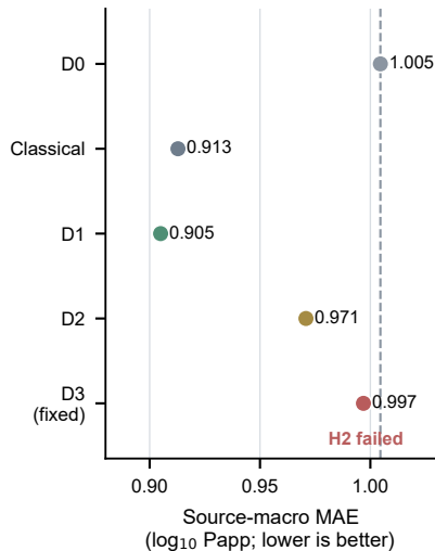
b Fixed D3 does not close the joint-block gap
