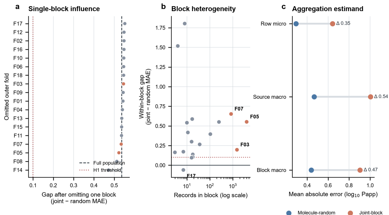
Supplementary Figure S1 | H1 influence and aggregation sensitivity. a , The D0 source-macro mean absolute error (MAE) gap between joint-block and molecule-random evaluation after omitting each of the 18 frozen joint blocks in turn. Points are ordered by the recalculated gap and labelled by the omitted outer fold. The black dashed line marks the full-population gap (0.537 \log_{10} Papp units), and the red dotted line marks the preregistered 0.10 point-gap threshold. Orange points identify omission of one of the three largest blocks. b , Within-block source-macro gap versus frozen block record count for all 18 blocks. The three largest blocks and the sole block with a negative within-block gap are labelled. The x axis is logarithmic; the red dotted line marks a gap of 0.10. c , Five-seed mean D0 MAE under row-micro, source-macro and equal-block-macro aggregation. Blue and orange points denote molecule-random and joint-block evaluation, respectively, and connecting segments show the corresponding gap. All panels use the already frozen 6,895-record, 41-source prediction population across five scheduled seeds. These post-confirmatory analyses involved no refitting or model selection and are descriptive; the original block/seed bootstrap remains the inferential H1 analysis.
