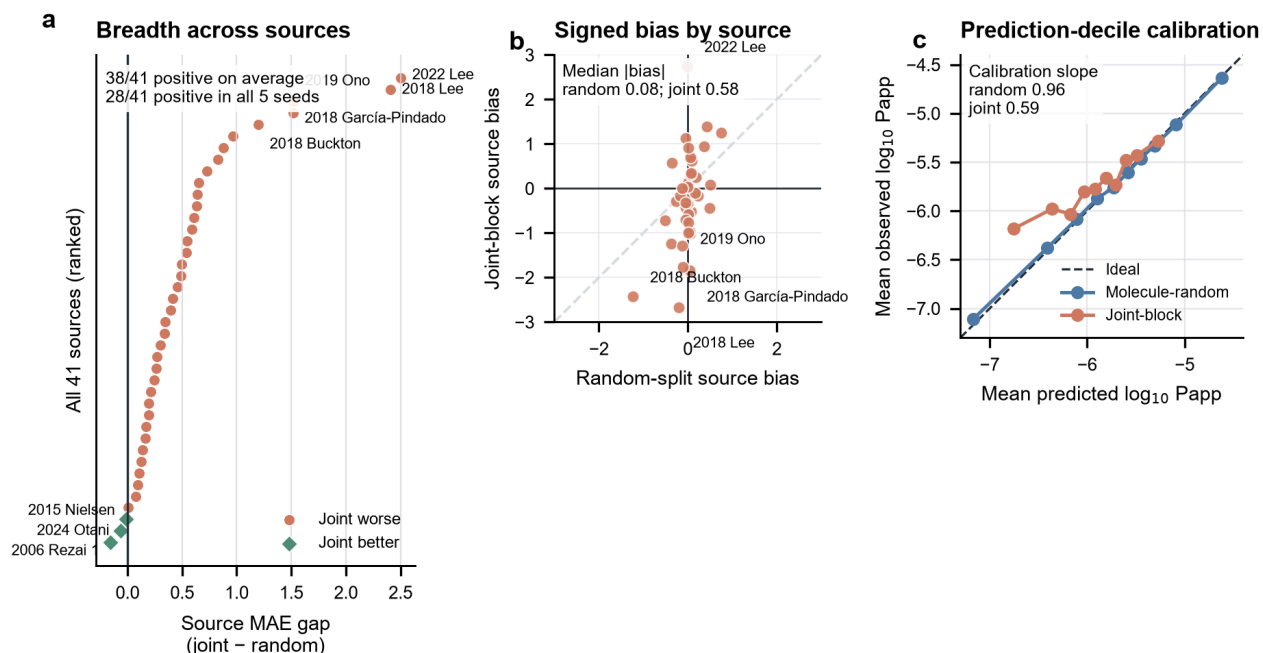
Supplementary Figure S2 | Source-stratified error and point-prediction calibration. a , Ranked source-level D0 MAE difference between joint-block and molecule-random evaluation for all 41 frozen sources. Orange circles indicate a higher joint-block MAE and green diamonds indicate a lower joint-block MAE; labelled points are the five largest positive differences and all three negative differences. Source summaries are means across five scheduled seeds. b , Five-seed mean signed error for each source under molecule-random and joint-block evaluation. Positive values indicate predicted permeability that is too high and negative values indicate predicted permeability that is too low. The dashed diagonal indicates equal bias under the two evaluation schemes; the five largest absolute joint-block biases are labelled. c , Point-prediction calibration after averaging the five frozen OOF predictions for each of 6,895 records. Points show mean observed versus mean predicted \log_{10} Papp within ten equal-frequency, arm-specific prediction bins; the dashed diagonal is ideal calibration. Slopes are from descriptive least-squares regressions of observed on mean predicted values. No refitting, recalibration or model selection was performed. Source data are provided as CSV files.
