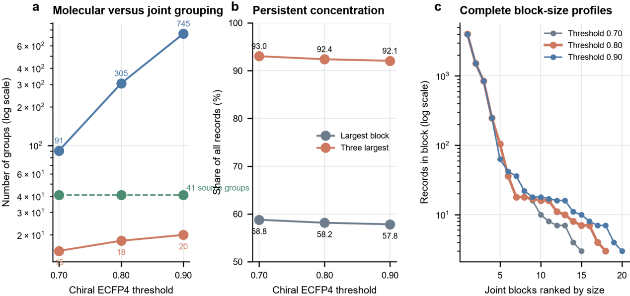
Supplementary Figure S3 | Analogue-threshold sensitivity of evidence geometry. a , Number of analogue components (blue) and source/component joint blocks (orange) reconstructed at chiral ECFP4 Tanimoto thresholds of 0.70, 0.80 and 0.90; the 41 source groups are shown as a green dashed reference. Counts use a logarithmic axis. The molecular-weight-ratio constraint, exact one-token cyclic-edit rule and source closure were held fixed. b , Percentage of all 6,895 records contained in the largest and three largest joint blocks at each threshold. c , Complete ranked joint-block size distributions on a logarithmic axis. The frozen primary threshold of 0.80 is emphasized in orange. Reconstruction used only public structure and provenance fields and exactly reproduced every primary 0.80 component/block identifier. No outcome, prediction or model-performance value was used. Alternative thresholds describe partition geometry only and were not used to rescore the frozen OOF predictions. Source data are provided as CSV files.
