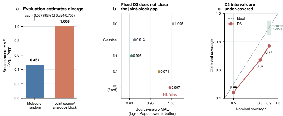
Fig. 3 Performance estimates and calibration across evaluation procedures. a , Source-macro mean absolute error (MAE; log 10 Papp) for the same D0 DMPNN under molecule-grouped pseudorandom and joint source/analogous-block evaluation. The annotated difference is joint-block minus molecule-grouped MAE; the 95% interval is the percentile interval from 10,000 paired outer-block/seed bootstrap replicates. Because the joint folds also changed the training-size profile, the contrast describes divergence between the two completed evaluation procedures rather than an isolated causal effect of dependence removal. b , Five-seed mean source-macro MAE under the joint-block protocol for D0, the nested-selected classical procedure, D1, D2 and the internally prespecified fixed candidate D3. Points show model means, and the dashed vertical line marks D0. Lower values indicate better prediction. D1 and D2 are secondary ablations and cannot replace D3 after outcome release. c , Nominal versus observed D3 empirical interval coverage across 34,475 frozen out-of-fold record-by-seed prediction slots (6,895 records x 5 seeds). Fold-local half-widths were computed from checkpoint-only inner-validation residuals using the finite-sample upper order statistic. The green segment marks the internally prespecified acceptable range (85-95%) for the nominal 90% interval. D3 achieves 77.0% slot-pooled coverage and is therefore under-covered; repeated seed slots are not independent experimental units. Source data are provided in the figure source-data directory.
