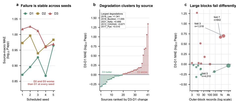
Fig. 4 Seed-stable but regime-dependent failure of the fixed D3 candidate. a , Source-macro MAE for D1, D2 and D3 across all five scheduled seeds. D2 and D3 are worse than D1 at every corresponding seed. b , D3-minus-D1 source-level MAE changes for all 41 sources, ranked from improvement to degradation. Values are five-seed means; green indicates lower error for D3 and red indicates higher error. The inset lists the five largest degradations. c , D3-minus-D1 block-level MAE change against the record count of every outer block on a logarithmic axis. Point area also represents record count. Folds 3 and 7 deteriorate strongly, whereas the largest block, fold 5, is slightly improved, demonstrating that failure is not a monotonic consequence of block size. Panels b and c are prespecified descriptive diagnoses and were not used to select a replacement model. Source data are provided in the figure source-data directory.
