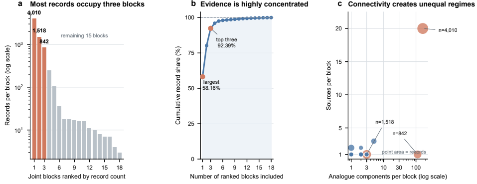
Fig. 2 Effective evidence geometry of the frozen joint blocks. a , Record counts for all 18 joint blocks, ranked from largest to smallest and shown on a logarithmic axis. Orange denotes the three largest blocks. b , Cumulative fraction of the 6,895 analytical records captured by the ranked blocks. The largest block contains 58.16% of records and the three largest contain 92.39%. c , Number of analogue components and contributing sources in each block. Point area represents the number of curated records, and the three largest blocks are labelled. All points represent frozen blocks; no jitter or simulated values were used. These panels describe the dependence structure of the dataset rather than a balanced target population. Source data are provided in the figure source-data directory.
