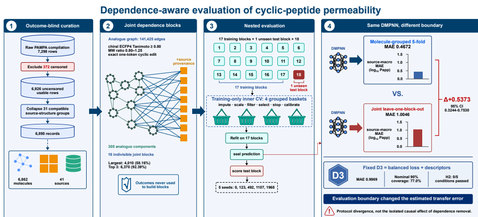
Fig. 1 Dependence-aware evaluation of cyclic-peptide permeability. 1. Outcome-blind curation of the cyclic-peptide PAMPA compilation. Of 7,298 raw rows, 372 carrying detection-limit annotations were excluded, leaving 6,926 uncensored usable rows. Median collapse of 31 compatible multi-row source-structure groups produced 6,895 analytical records representing 6,862 unique molecules from 41 sources. 2. Peptide-aware analogue relationships were closed transitively into 305 analogue components and combined with source provenance in a bipartite graph. Connected components produced 18 indivisible joint blocks; neither permeability values nor model errors were used to construct them. The largest block contained 4,010 records (58.16%) and the three largest contained 6,370 records (92.39%). 3. Each joint block served once as an unseen outer test block while the other 17 blocks formed the outer-training population. Imputation, scaling, filtering, selection, stopping and residual calibration were restricted to four training-only grouped inner baskets before refitting, prediction sealing and test-block scoring. 4. Under the completed molecule-grouped five-fold and joint leave-one-block-out procedures, the same D0 DMPNN had source-macro MAEs of 0.4672 and 1.0046, respectively; the joint-minus-molecule-grouped difference was 0.5373 (95% percentile interval, 0.3244-0.7530). The panel also summarizes the fixed D3 candidate (MAE 0.9969; nominal-90% slot-pooled interval coverage 77.0%; 0/5 H2 conditions passed). The comparison describes divergence between the two completed procedures and does not isolate the causal contribution of dependence removal from the changed training-size profile. Icons and block widths are conceptual and are not drawn to scale.
