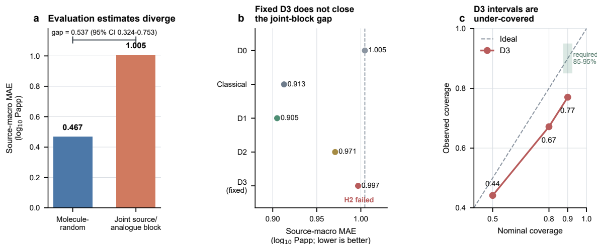
Figure 3: Performance estimates and calibration across evaluation procedures. a , Source-macro mean absolute error (MAE; log 10 Papp) for the same D0 DMPNN under molecule-grouped pseudorandom and joint source/analogue-block evaluation. The annotated difference is joint-block minus molecule-grouped MAE; the 95% interval is the percentile interval from 10,000 paired outer-block/seed bootstrap replicates. Because the joint folds also changed the training-size profile, the contrast describes divergence between the two completed evaluation procedures rather than an isolated causal effect of dependence removal. b , Five-seed mean source-macro MAE under the joint-block protocol for D0, the nested-selected classical procedure, D1, D2 and the internally prespecified fixed candidate D3. Points show model means, and the dashed vertical line marks D0. Lower values indicate better prediction. D1 and D2 are secondary ablations and cannot replace D3 after outcome release. c , Nominal versus observed D3 empirical interval coverage across 34,475 frozen out-of-fold record-by-seed prediction slots (6,895 records x 5 seeds). Fold-local half-widths were computed from checkpoint-only inner-validation residuals using the finite-sample upper order statistic. The green segment marks the internally prespecified acceptable range (85-95%) for the nominal 90% interval. D3 achieves 77.0% slot-pooled coverage and is therefore under-covered; repeated seed slots are not independent experimental units. Source data are provided in the figure source-data directory.
