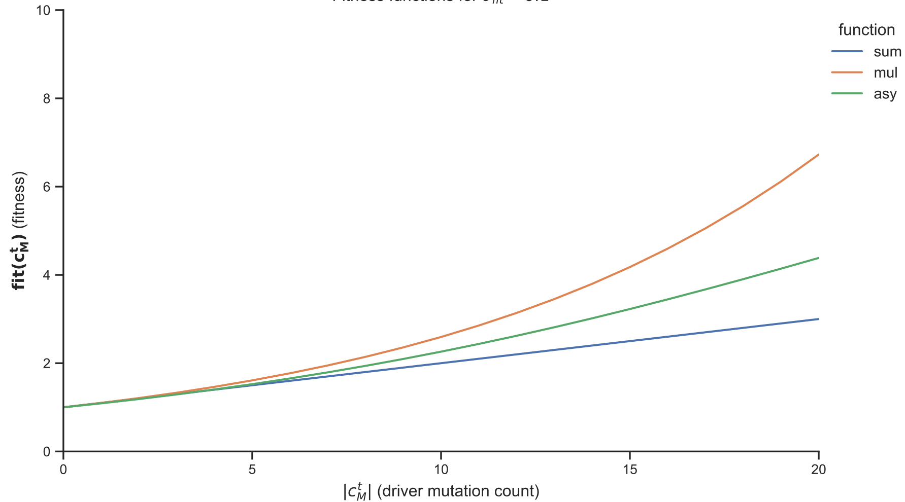
Fitness functions for \theta_{fit} = 0.1
