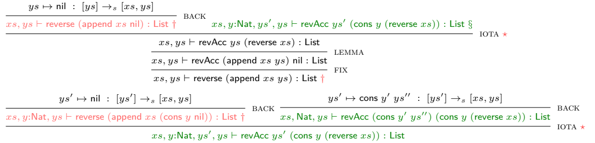
Fig. 1. Cyclic proof for reverse (append xs ys) . \dagger = companion (all backlinks point here). FIX : unfold reverse . LEMMA : LLM cut revAcc (append xs ys) acc = revAcc ys (revAcc xs acc) , validated by sub-prover. IOTA : case on ys (top) or ys' (bottom). BACK : the nil branch (at any depth) is an instance of the root companion under a suitable substitution: ys \mapsto \text{nil} (top), ys \mapsto \text{cons } y \text{ nil} (bottom). The cons branch repeats the pattern; termination by structural induction on the cons chain (every split removes one cons ).
