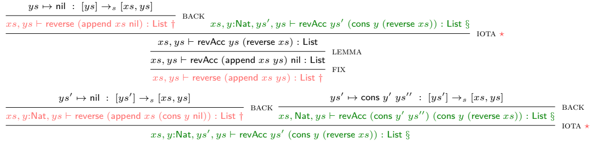
Fig. 1. Cyclic proof for reverse-append fusion.
