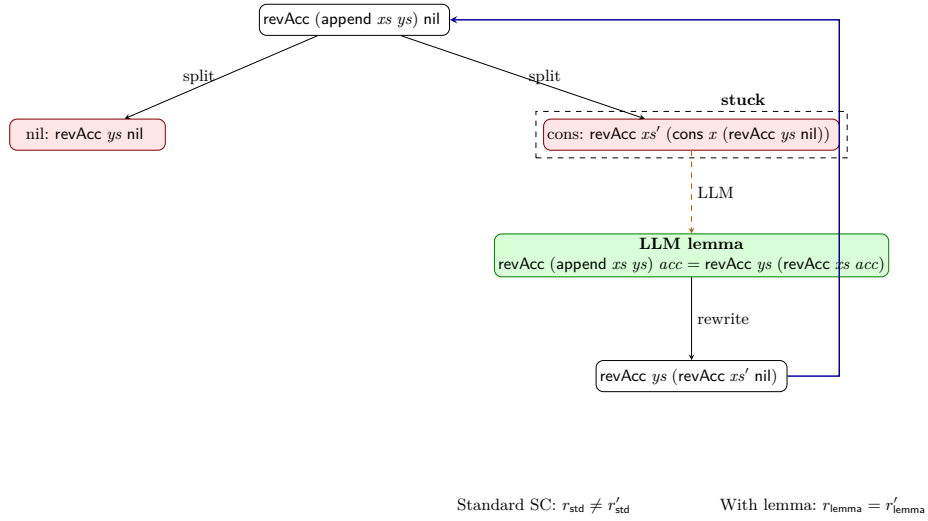
Fig. 1. Cyclic proof graph for reverse-append fusion. The standard SC gets stuck at the cons branch (red); the LLM proposes a lemma (green) that rewrites the stuck configuration into a form that folds (blue backlink) to the root. Without the lemma, standard SC produces different residuals for the two sides of the equation; with the lemma, the residuals are identical.
