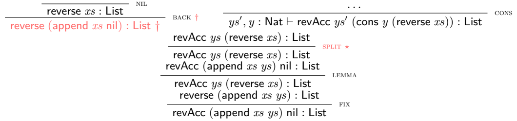
Fig. 5.11. Cyclic proof for reverse-append fusion. Red = companion (backlink target); \dagger = backlink; \star = progress event; LEMMA = LLM cut; FIX = unfold reverse. The nil branch closes via BACK; the cons branch ( \dots ) drives further and folds to the root through induction on ys .
