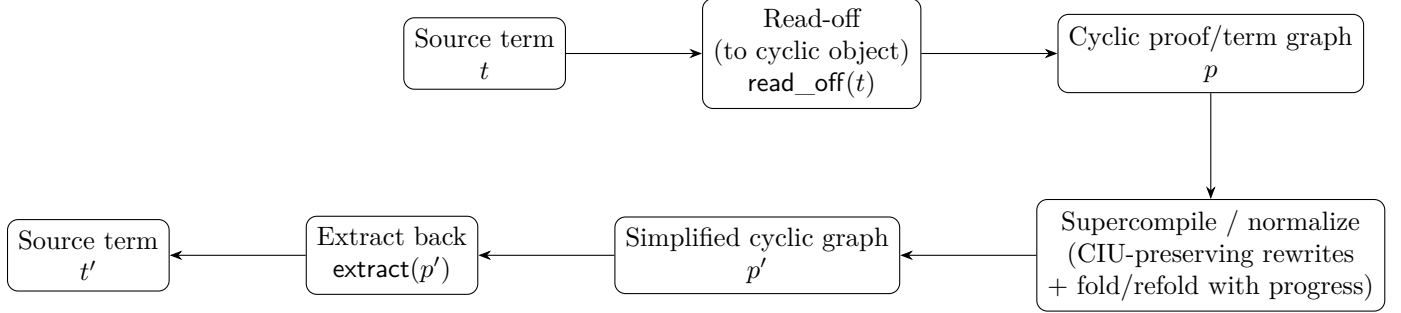
Figure 1: Normalization pipeline: compile terms to cyclic objects, simplify by supercompilation, then extract back to term syntax. The intended equality notion is t \approx t' up to typed CIU, and fold/refold steps are constrained by global progress evidence.
