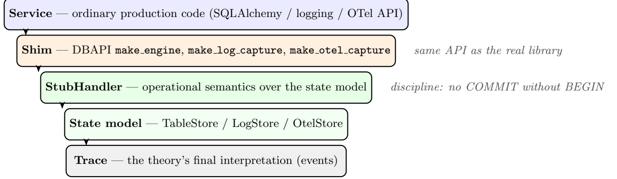
Figure 4: The theory stack. The service is written once, against the real library API; the shim connects that API to the stub; the stub interprets actions over a pure state model and records the trace. Differential tests run the same programs against stub and real library and require identical observable behaviour.
