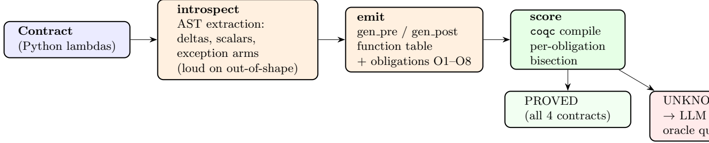
Figure 5: The lowering pipeline: introspect, emit, score.
