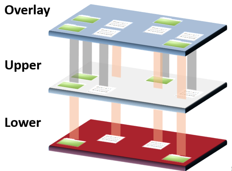
Figure 1: Visual Representation of Layers in an Overlay Filesystem
