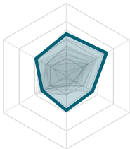
5. qlattice (30.6)
