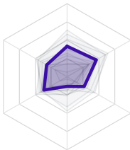
10. tpsr (21.3)
