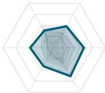
5. qlattice (30.6)
