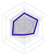
10. tpsr (21.3)
