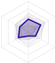
10. tpsr (21.3)
