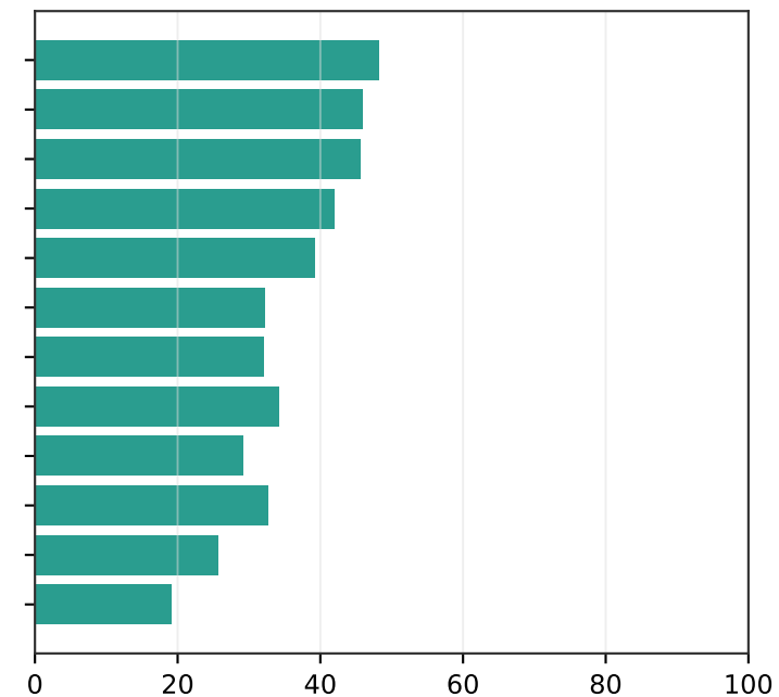
STAB
