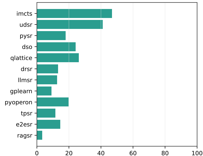
EFF
