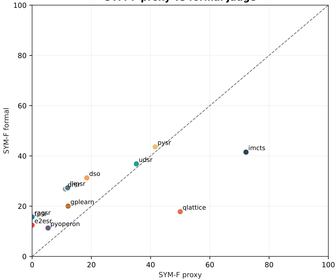
SYM-F proxy vs formal judge
