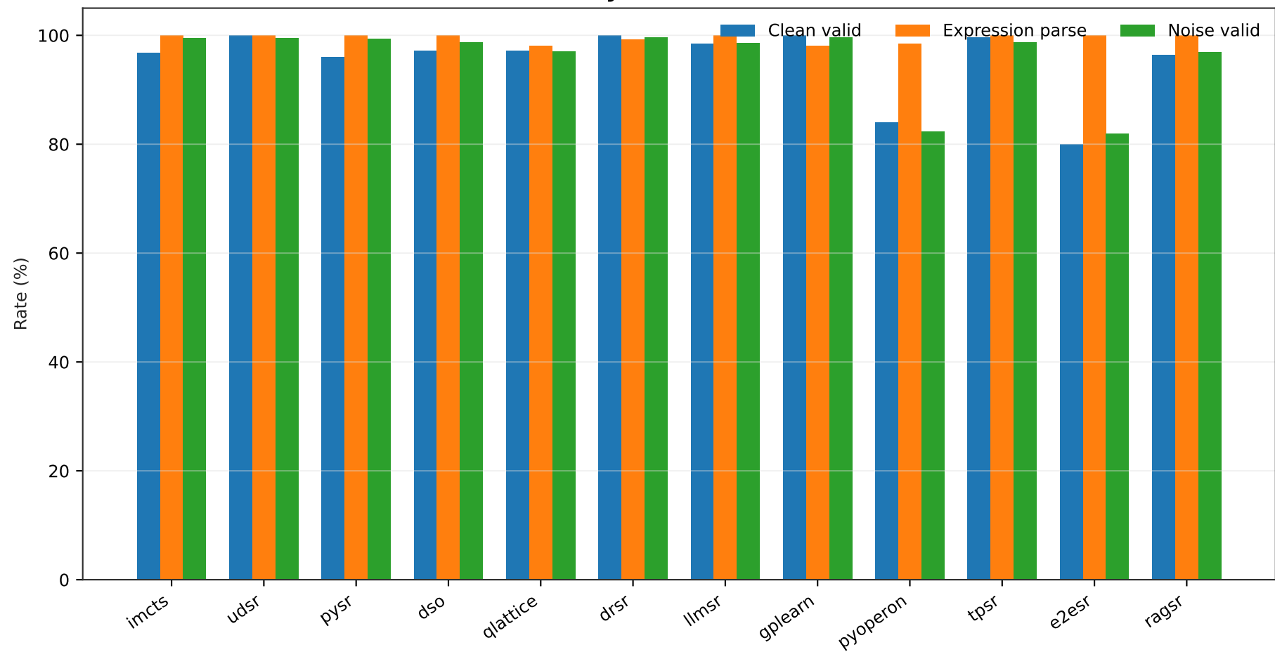
Validity and Parse Rates
