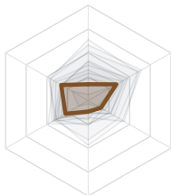
10. tpsr (21.3)
