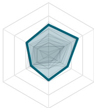
5. qlattice (30.6)
