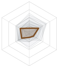
10. tpsr (21.3)
