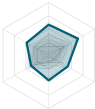
5. qlattice (30.6)
