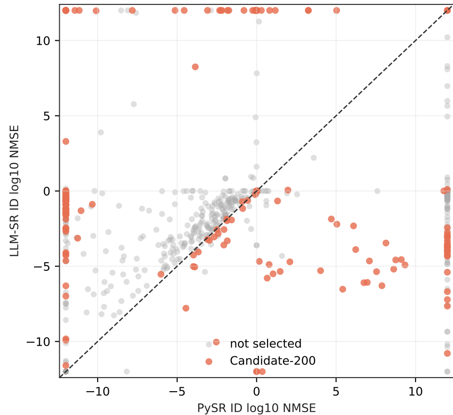
ID probe disagreement
