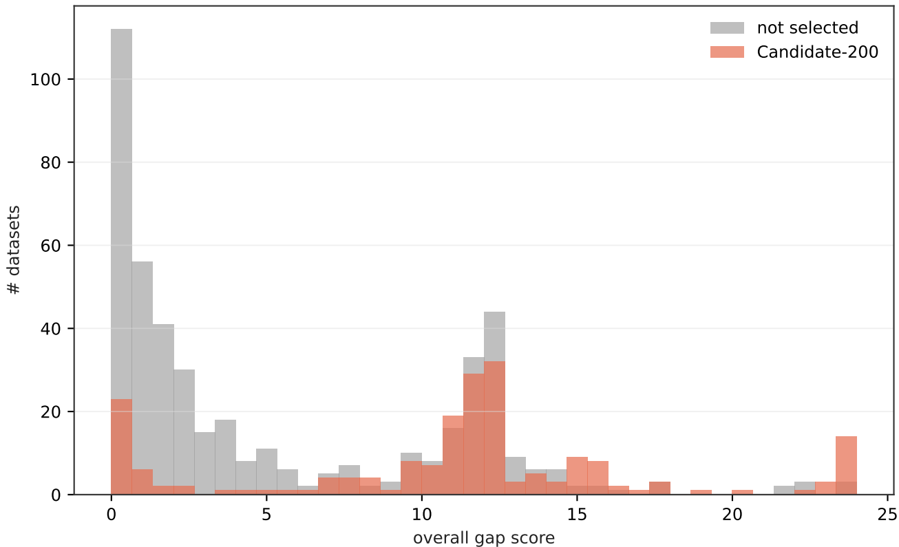
Candidate-200 shifts toward high-disagreement tasks
