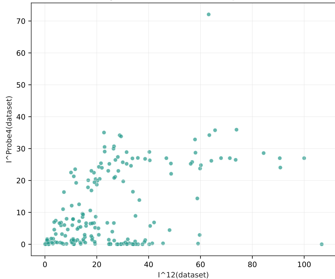
Panel fidelity on Candidate-200 (Spearman=0.369)
