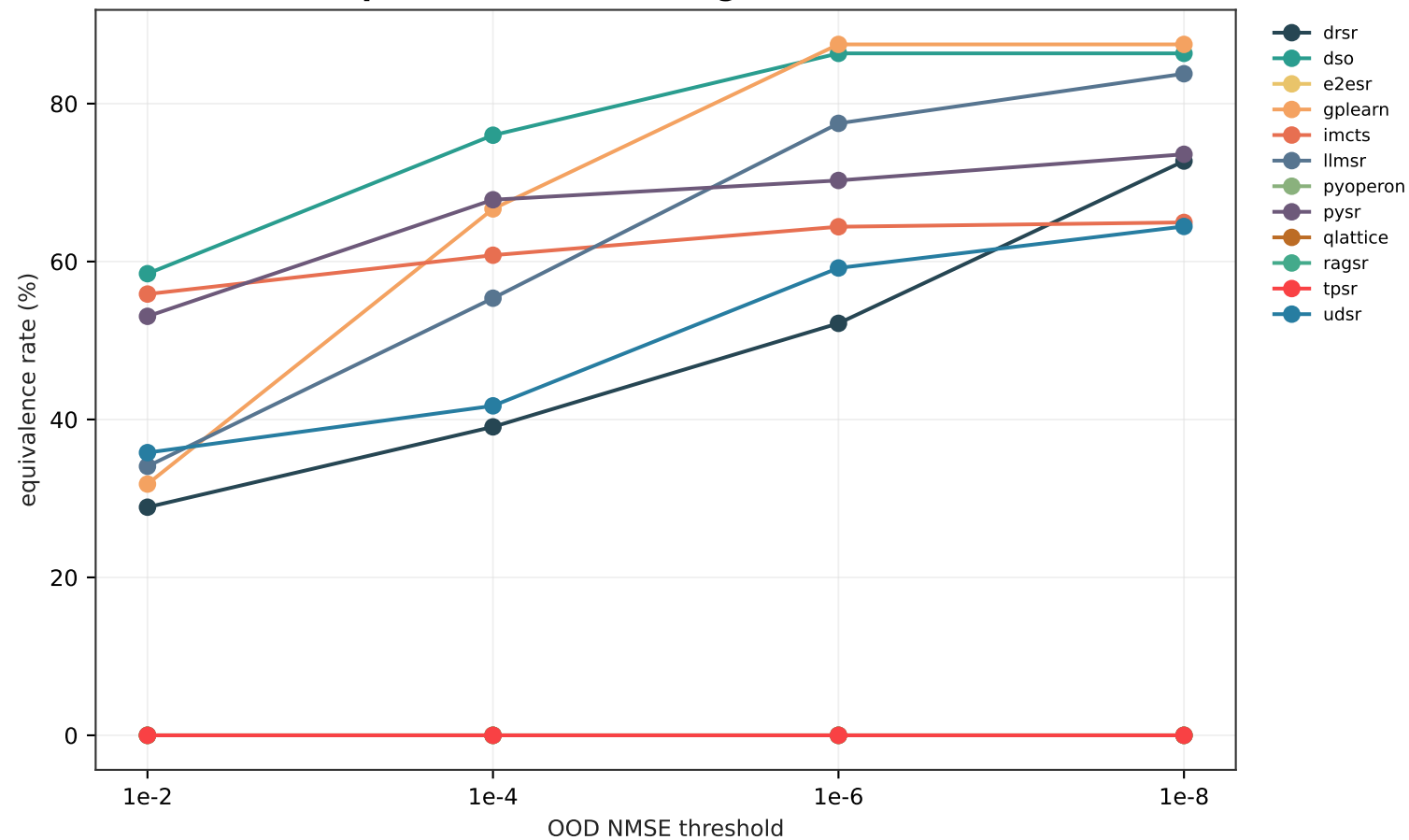
Equivalence rate among low-NMSE runs
