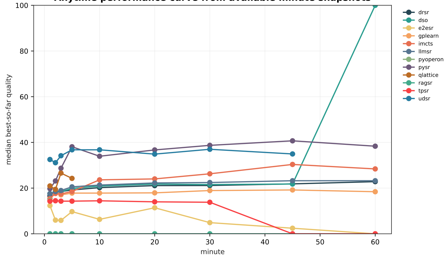
Anytime performance curve from available minute snapshots
