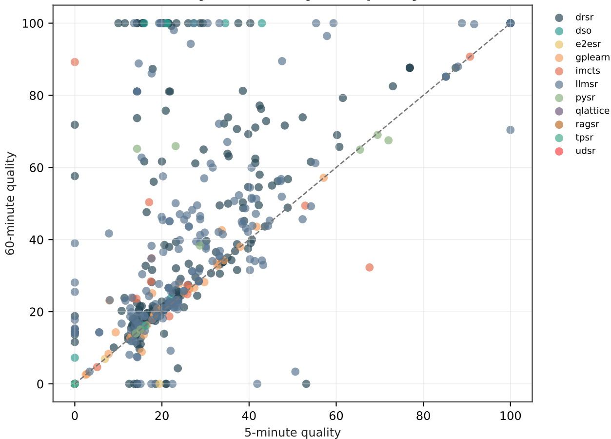
Early vs final anytime quality
