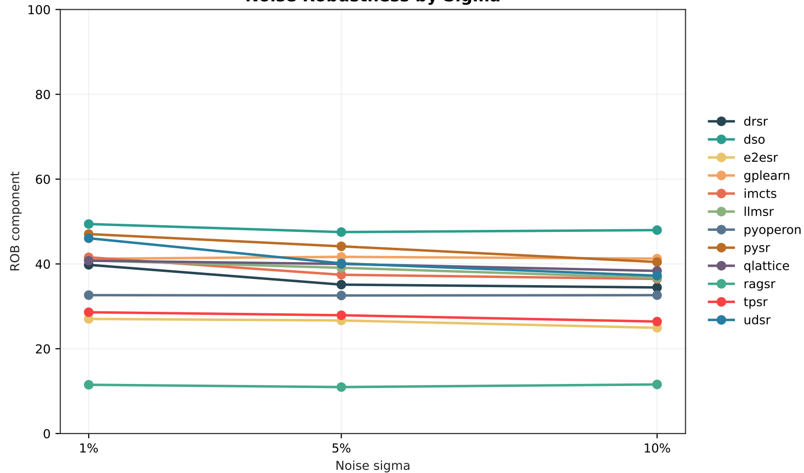
Noise Robustness by Sigma
