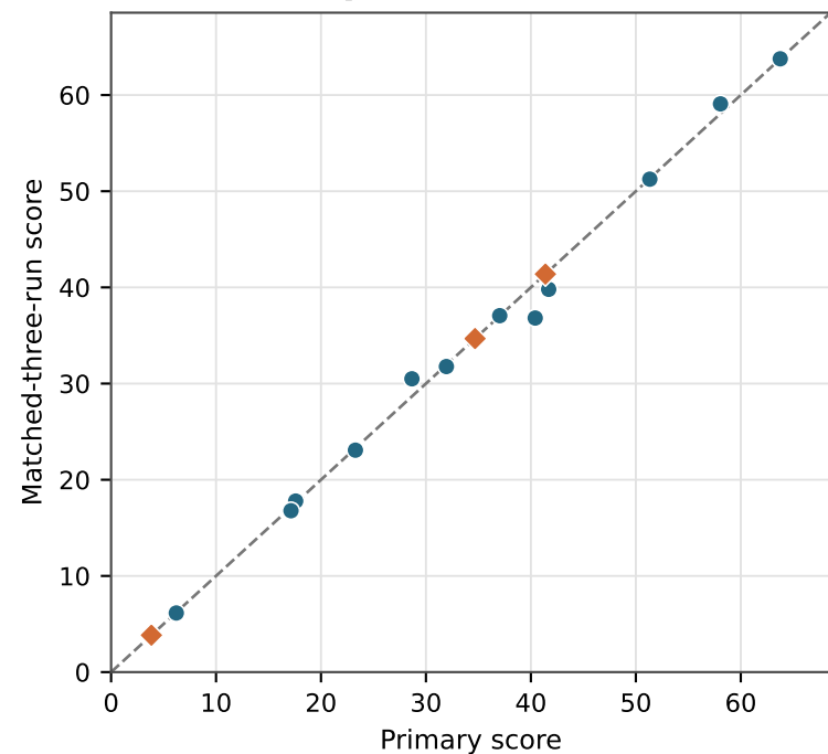
ID-Q (rank r=0.993 )
