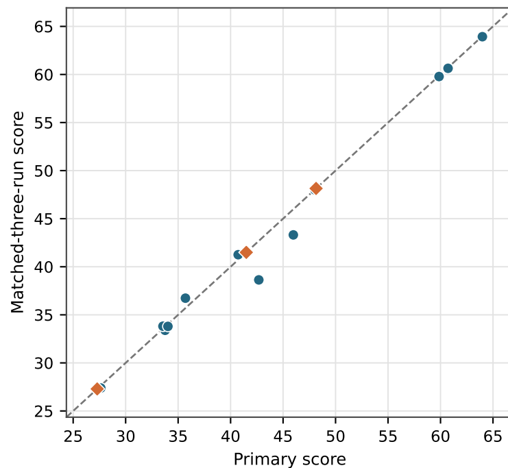
OOD-G (rank r=0.979 )
