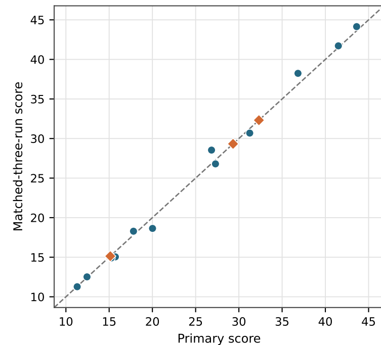
SYM-F (rank r=0.986 )
