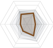
10. tpsr (21.3)
